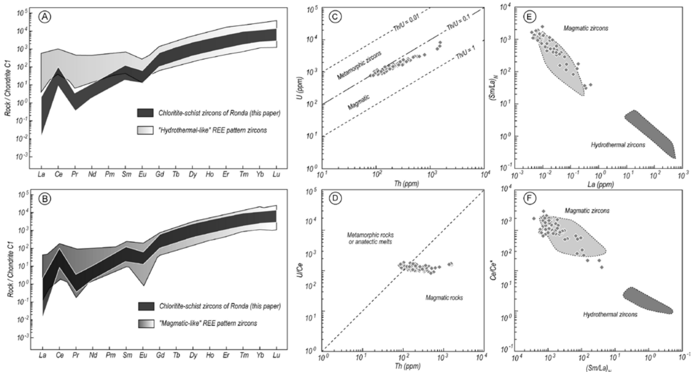
Fig. 3.- Comparative normalized REE diagram (C1 Chondrite; McDonough and Sun, 1995) of chlorite schist zircons to "hydrothermal" (A) and "magmatic-like" (B) hydrothermal zircon crystals. U vs. Th (C), U/Ce vs. Th (D), (Sm/La) N vs. La (E) and Ce/Ce* vs. (Sm/La) N (F) discrimination diagrams for metamorphic, hydrothermal and magmatic zircon crystals.
