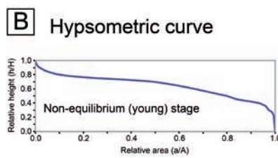
Fig. 3. A) Licus Vallis basin and stream ordering according to Strahler's classification. 1: Impact crater with a possible paleolake that eventually overflowed; 2: Channel interrupted by impact craters. B) Hypsometric curve of the basin. C) Smoothened profile of the main channel. See color figure in the web.
