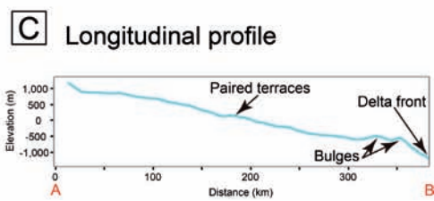
Fig. 3. A) Licus Vallis basin and stream ordering according to Strahler's classification. 1: Impact crater with a possible paleolake that eventually overflowed; 2: Channel interrupted by impact craters. B) Hypsometric curve of the basin. C) Smoothened profile of the main channel. See color figure in the web.
