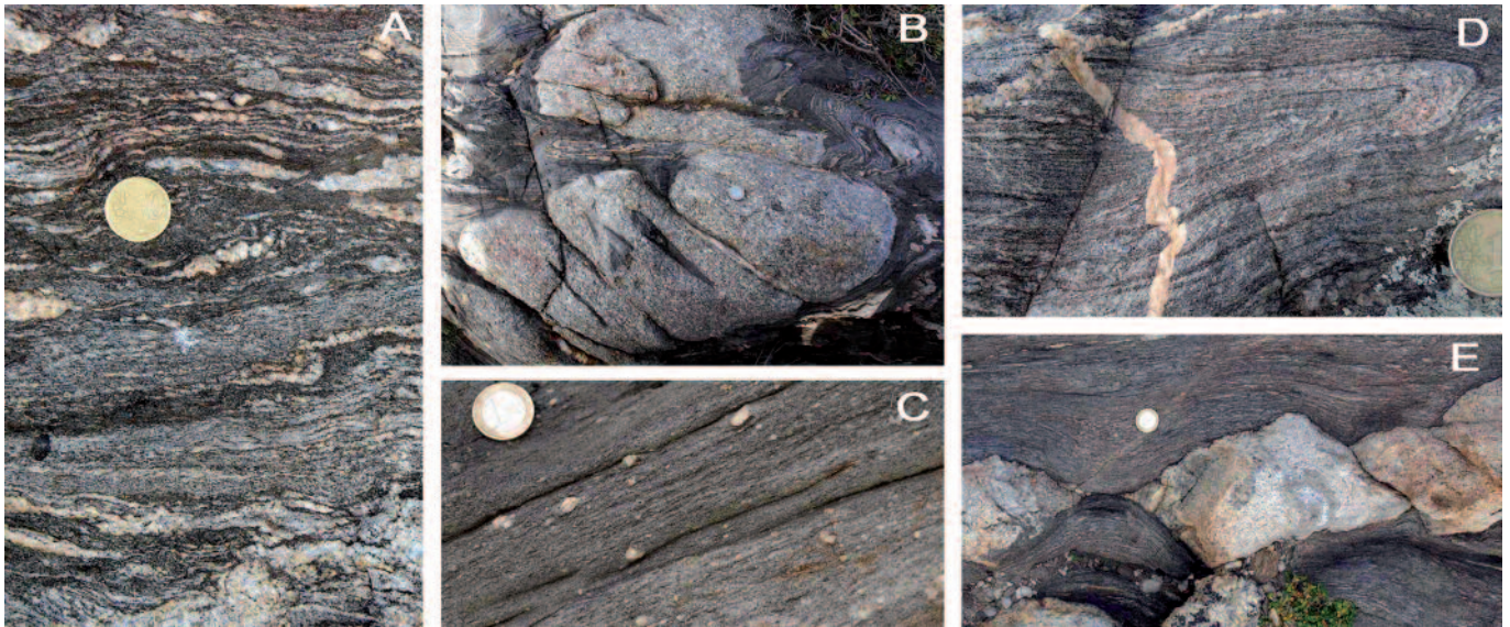
Fig. 2.- Field photographs from the study area in South Volt Andrau. A) Stromatic migmatite with differentiated leucosome, melanosome and mesosome layers. Layering is parallel to S_2 foliation. B) Folded sub-tabular granodiorite body showing an internal axial planar S_2 foliation. C) Detail of S_2 gneissic foliation in a porphyritic granodiorite. Feldspar phenocrysts are surrounded by the deformed matrix. D) A D_2 syntectonic leucogranite vein cross-cuts the folded schists. Both are coplanarly folded with a marked difference in strain: tight folds in the schists and open folds in the vein. E) Asymmetrically boudinaged leucogranite dyke. Boudins are delimited by dextral shear fractures.
