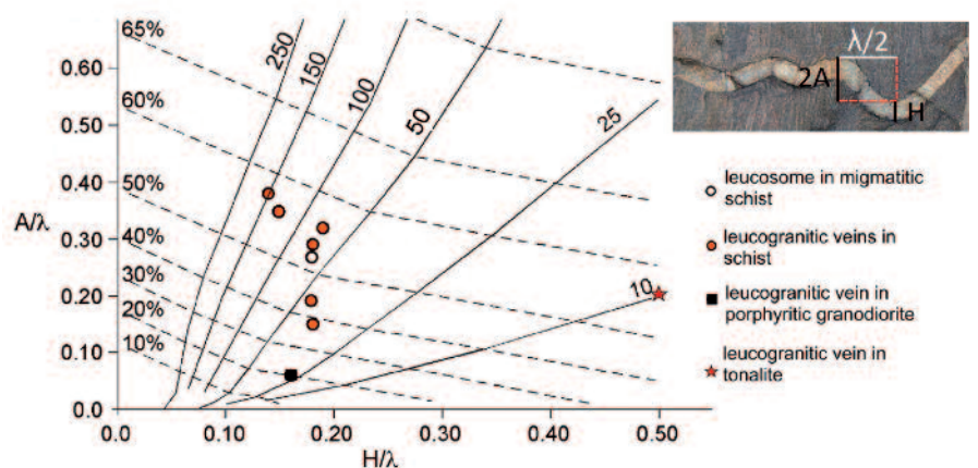
Fig. 3.- Ratios of A/\lambda and H/\lambda from measured fold profiles in leucocratic veins plotted in the strain contour map of Schmalholz and Podladchikov (2001). The solid lines refer to the competence contrasts and the dashed lines to the percentage of vein shortening.
