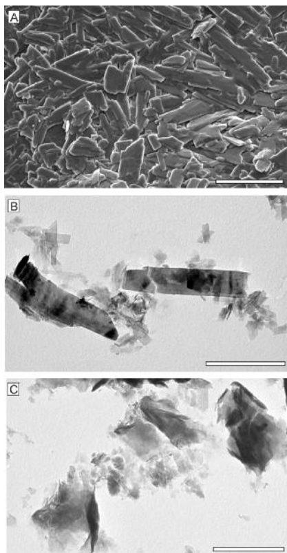
Fig. 4.- Electron microscopy images. A) Lath-like crystals of glauconite (SEM). B) Lath-like crystals of glauconite (TEM). C) Veil-like grains of smectite (TEM). Scale bar 1 \mu m.
