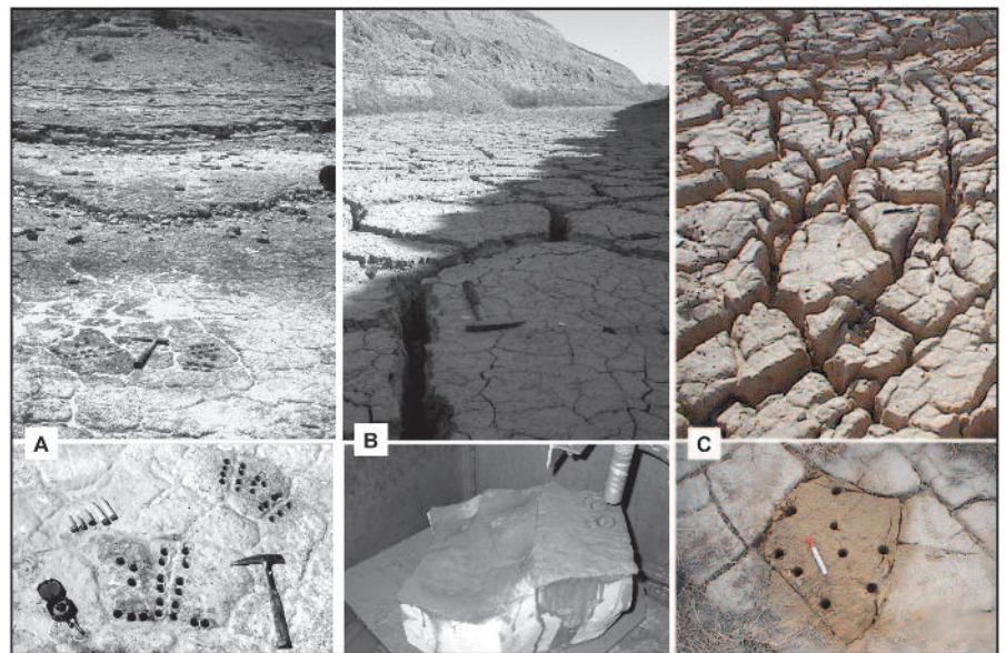
Fig. 1.- Field aspects of the sampled sites. A) Cracks in upper Miocene lacustrine limestones (Ebro Basin, Spain). Site MC01. B) Decimetric-scale mud cracks in recent flood plain marls. Site MC02. C) Cracks in fine grain-size detrital material linked to anthropic disposal. Site MC03.
