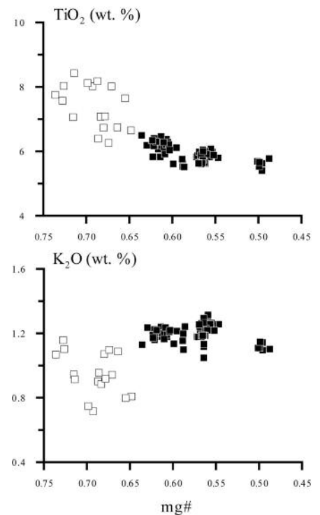
Fig. 3.- Top: TiO 2 vs mg# diagram for Krs megacrysts. Bottom: K 2 O vs mg# diagram. Black squares: megacryst cores; white squares: megacryst rims.
