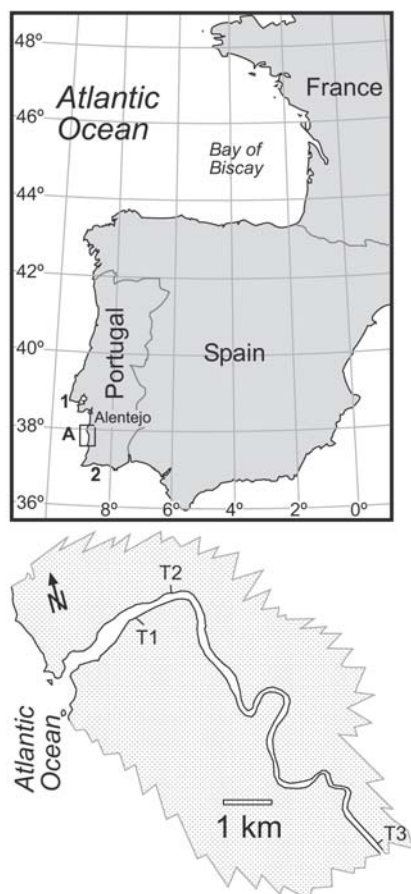
Fig. 1.- Geographical location of the study area. Location of the most relevant tide gauges is also indicated. Key: 1- Cascais; 2- Lagos; A- Mira estuary; T1-T3: Transects.
