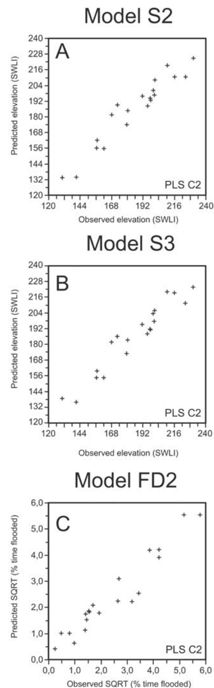
Fig. 2.- Observed and predicted values of the SWLI for Models S2 and S3 (component 2) and observed and predicted values of the % SQRT flooding time for Model FD2 (component 2) of the foraminiferal transfer functions.
