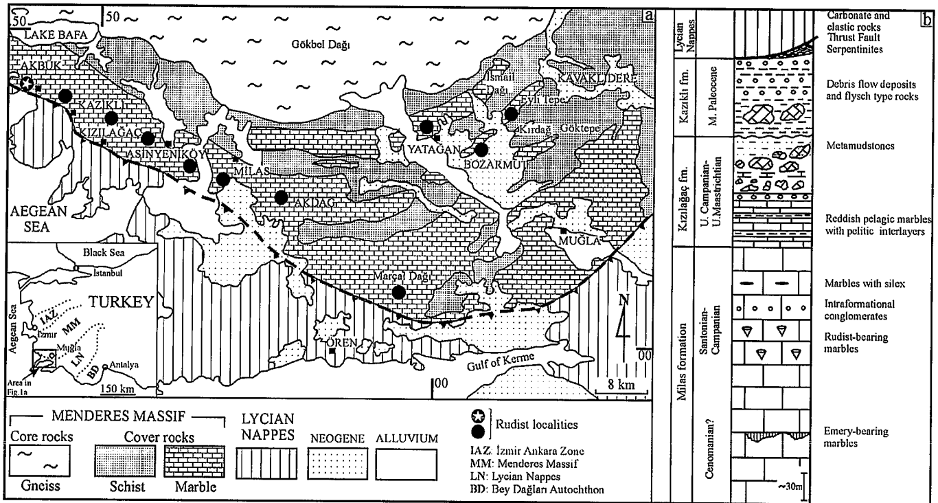
Fig. 1.- a) Geological map of the southern Menderes Massif with indication of rudist localities (modified from Dürr, 1975; Çağlayan et al. , 1980 and Konak et al. , 1987); b) Generalized stratigraphic section of the Akbuk area (after Özer et al. , 2001).
