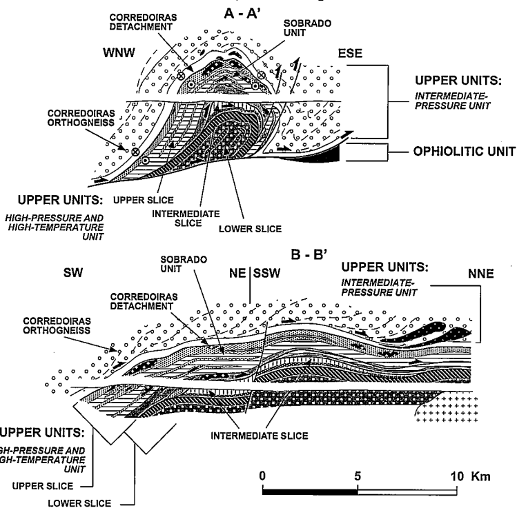
Fig. 3.- Transverse (A-A') and longitudinal (B-B') sections across the Sobrado tectonic window. See location in Fig. 2. Note "top-to-the-NE" sense of motion of the Corredoiras Detachment (section B-B'), and subsequent SE-directed thrusting (section A-A').
