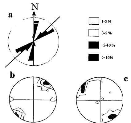
Fig. 4. Dykes in Yanci-Aranaz sector. a) Rose diagram of dyke directions. b) Density plot for main phase fold axes. c) Density plot for main phase cleavage poles (b and c, after Martínez-Torres & Ramón-Lluch, 1984).
