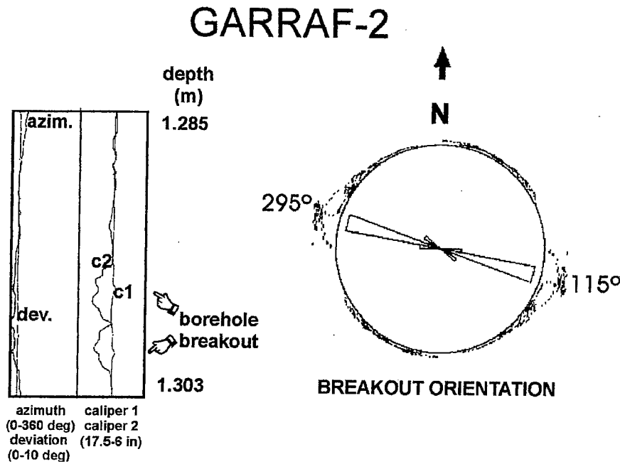
Fig. 1.- Borehole breakout example from the Garraf-2 well (Mediterranean offshore, NW Valencia Trough). On the left, the caliper and the orientation logs (azimuth and deviation) for the depth interval 1285-1303 m. Two aligned breakouts show up in the caliper logs. A maximum caliper difference of about 3 inches (7.32 cm) and over a depth interval length of about 7 m. The smoothly varying deviation curve shows the deviation of the well from the vertical. The azimuth curve shows the orientation of the tool reference pad in the well. The tool rotates as long as both caliper diameters do not differ significantly. The contour-plot on the right is the projection of the caliper and represents the stack of the caliper data for the depth interval 1285-1303 m. The breakouts are observed to occur in this case at azimuths of 115° and 295° with respect to magnetic North indicating an orientation of S_H = N 25^\circ E .
