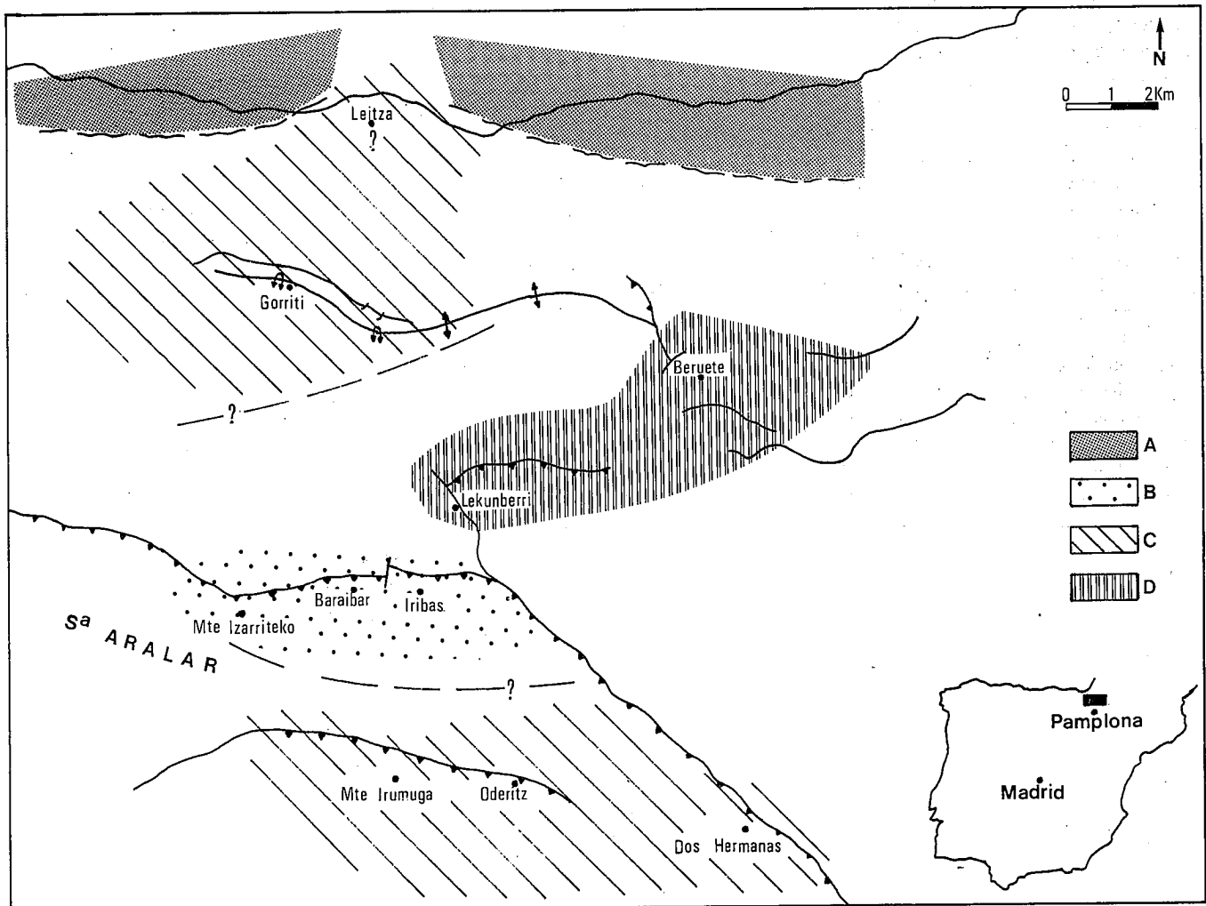
Fig.1.— Location map showing the recorded sections and the facies distribution during the Late Bajocian (Subfurcatum Zone). Legend: A: unit eroded, B: sponge boundstone and floatstone, C: grain-supported facies (tuberolitic and bioclastic packstone), D: micritic facies bearing ammonites and scarce sponge debris.
