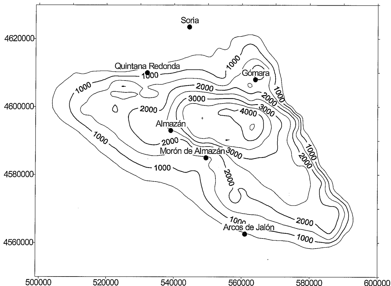
Figure 2.- Tertiary and Upper Cretaceous isopach map. Contour interval 500 m. UTM coordinates in metres, huse 30.
