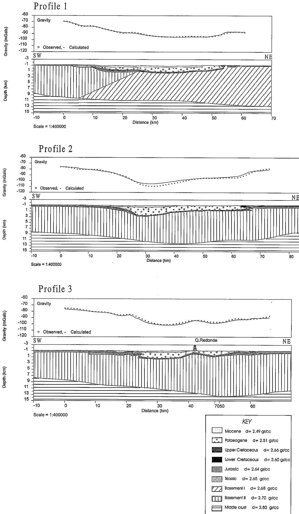
Figure 9.- 2+1/2 D gravity models representing the boundary between basement and middle crust as well as surface geology and basin geometry as deduced from seismic data. No vertical exaggeration.
