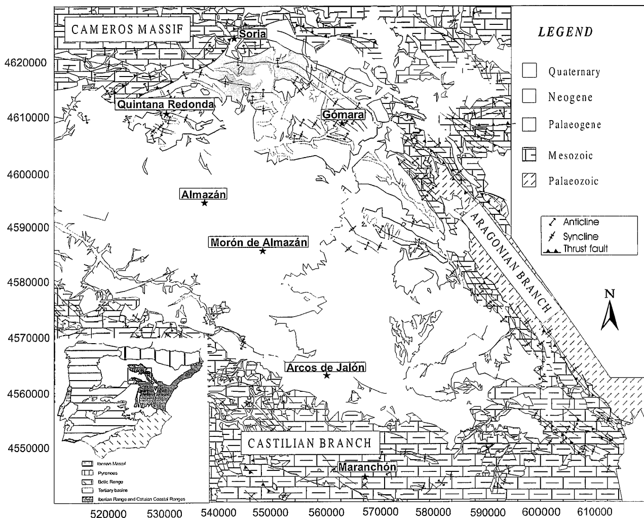
Figure 1.- Geological map of the Almazán Basin and location of the Almazán Basin within the Iberian peninsula. UTM coordinates in km. Huse 30.
