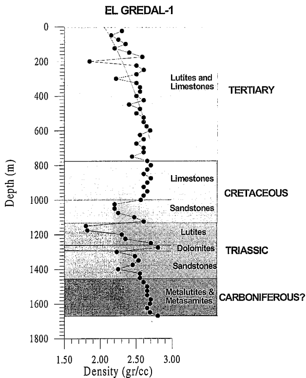
Figure 5.- Density log derived from El Gredal well. See location on figure 3. Black line between 0 and 700 m depth represents the least square fit to a quadratic function for depth variation density. The density obtained has been used for the computation of the gravity anomaly depicted on figure 4.
