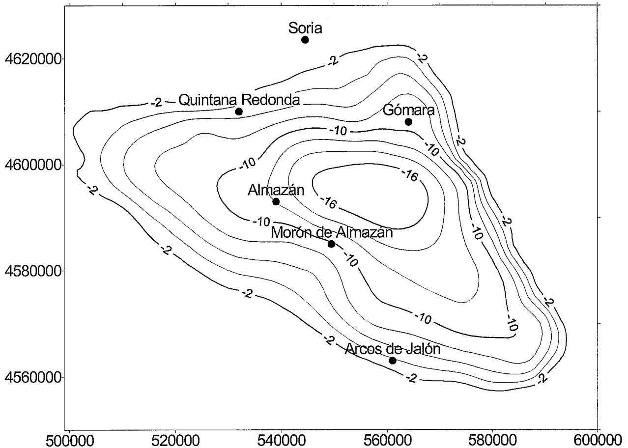
Figure 4.- Theoretical gravity anomaly map, showing the gravity effect of the sedimentary infill, using a density ranging at depth from 2.46 gr/cc to 2.69 gr/cc. Interval 2 mGal. UTM coordinates as in figure 2.
