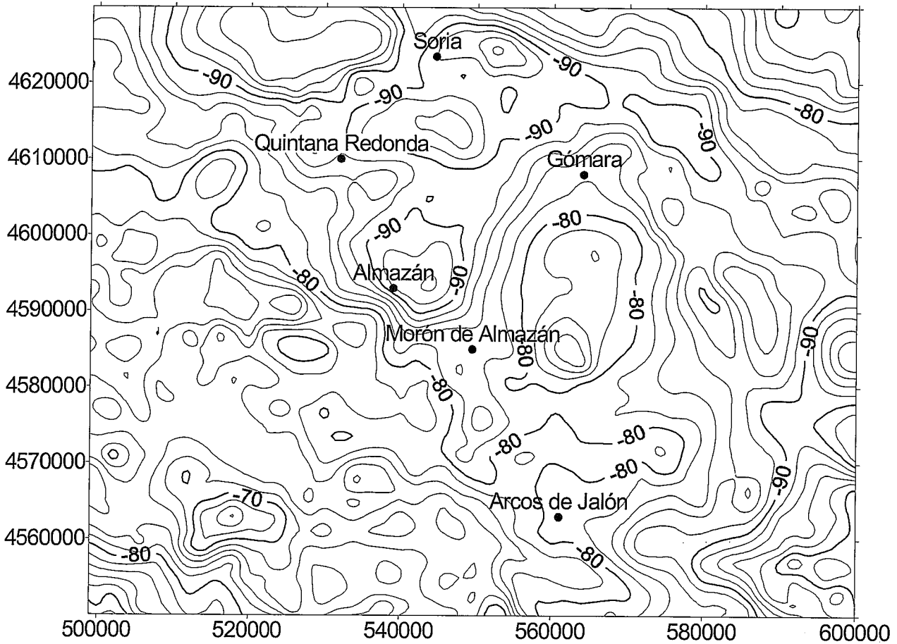
Figure 6.- Theoretical gravity anomaly map obtained by subtracting the gravity anomaly map due to the sedimentary infill from the observed gravity anomaly map. Contour interval 2mGal. UTM coordinates as in figure 2.
