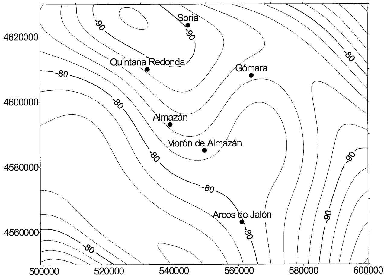
Figure 8.- Bouguer anomaly map showing the effect of the regional source isolated. Contour interval 2 mGal. UTM coordinates as in figure 2.
