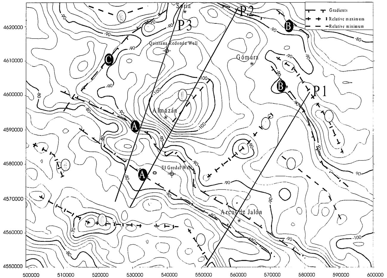
Figure 3.- Gravity anomaly map of the Almazán Basin. Contour interval 2 mGal. UTM coordinates as in figure 2. The location of the three gravity models is shown. Numbers and letters refer to features described on the text.
