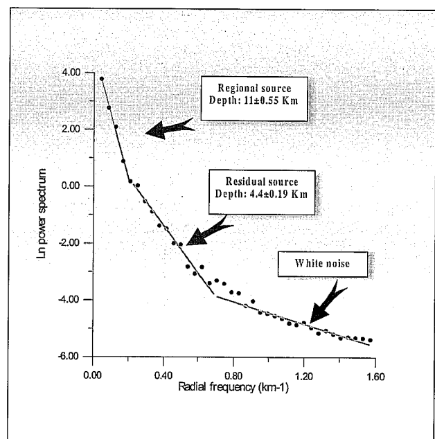
Figure 7.- Graph showing power spectrum versus radial frequency for the gravity map in figure 3. Three different sources, regional, residual and white noise are distinguished, and their mean depths have been calculated.
