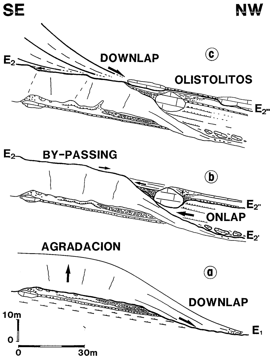
Fig. 3.—Detailed facies relationships of the Aldabide tongue and related sediments. Note the erosional base and top of the bioherm and the olistolith accumulation in front of the tongue (basinwards).
