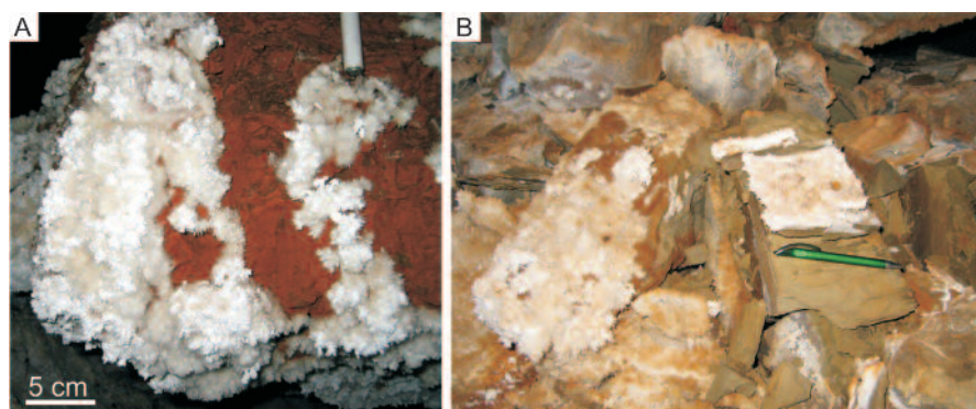
Fig. 2.- Speleothems containing Mg minerals. A) Moonmilk globules covering aragonite frostworks that nucleate on red soil of the cave. B) Polymineral crust speleothems covering fragments of shales.
