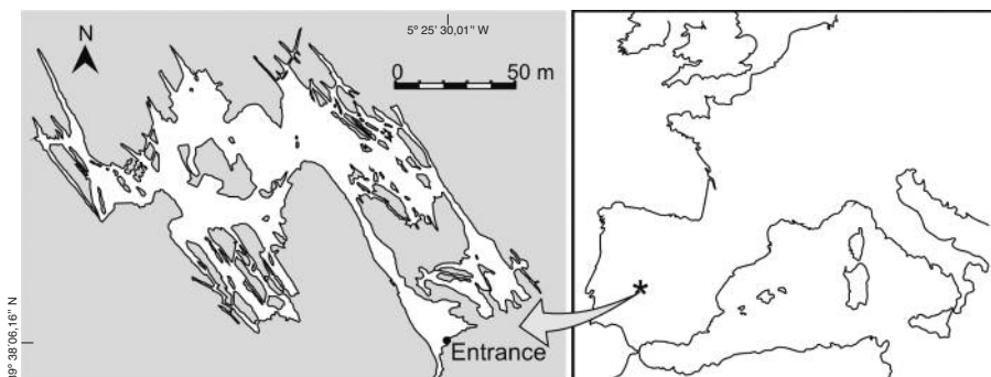
Fig. 1.- Castañar cave map and location of Castañar in Iberian Peninsula.
